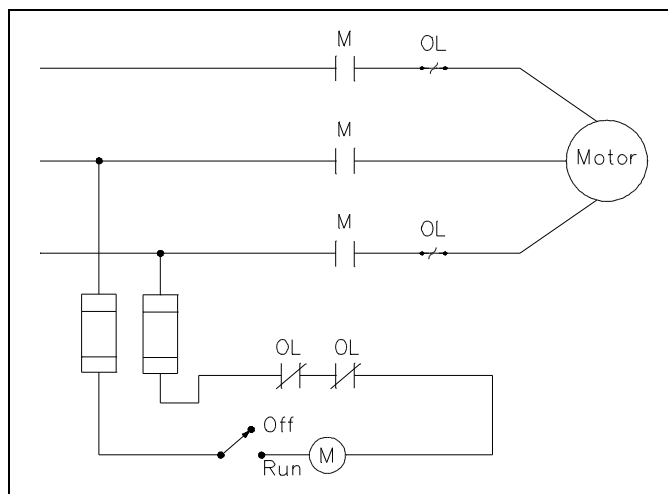
Figure 13 LVR Controller
