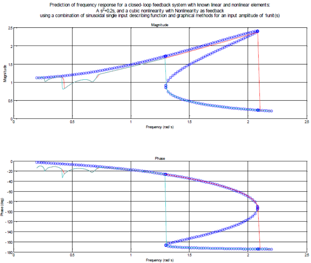
Figure 5.13 Swept frequency response test for c = 0.2 compared with the theory.
