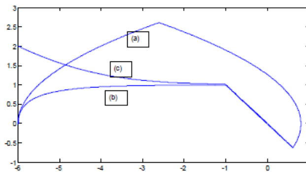
Figure 9.9 Phase plane responses for the two different control laws.
