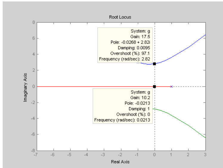
Figure 4.5 Root locus plot for transfer function of equation (4.7)
